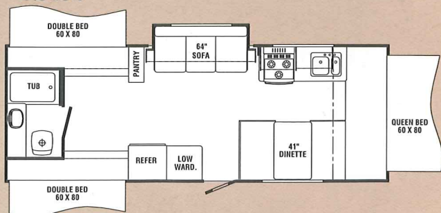
C243S
